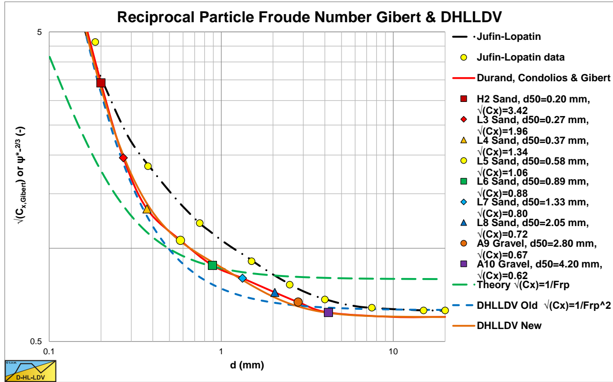
Figure 5-5: The reciprocal particle Froude number of Jufin-Lopatin, Gibert and DHLLDV.
