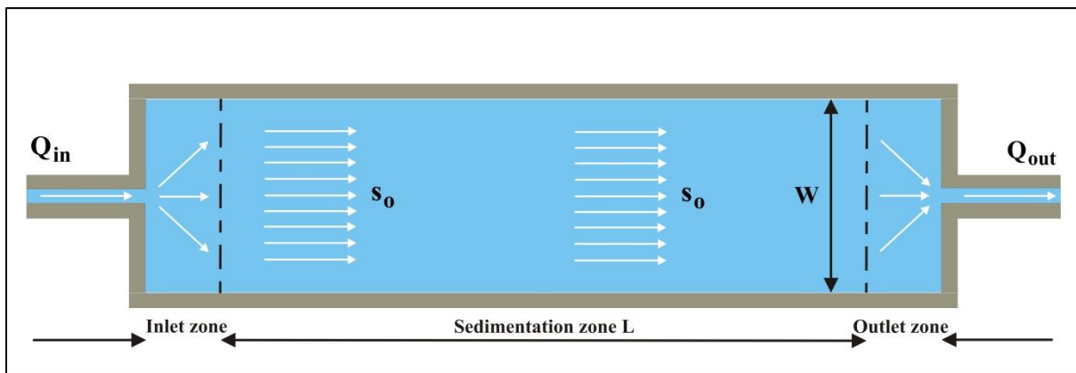
Figure 8-19: The top view of the ideal basin.
